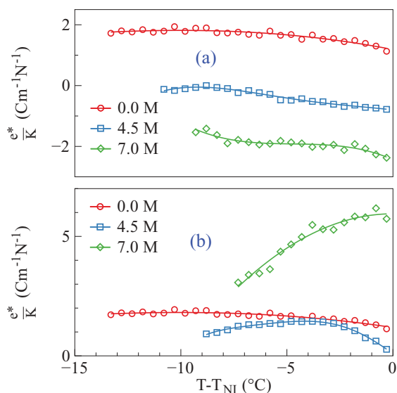
FIG. 4. (Color online) Temperature variation of flexoelectric ratio e^*/K for (a) mixtures with BC-120 and (b) mixtures with BC-60 molecules for three different concentrations, 0, 4.5, and 7M%. Continuous lines are drawn as guides to the eye.
